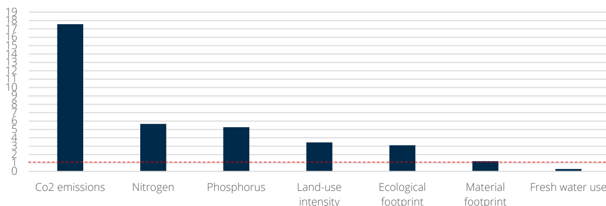
Figure 1: ROI per capita consumption relative to respective boundary (=1)
